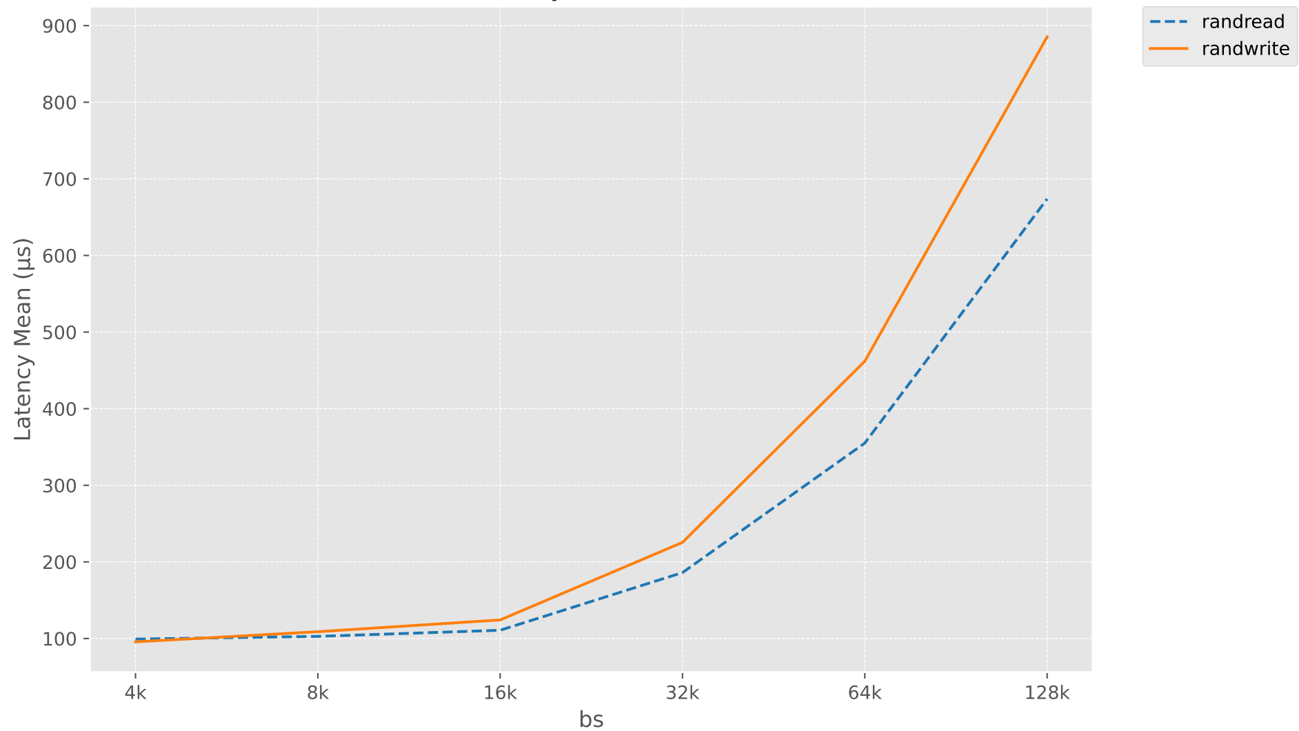
Latency Mean vs bs
